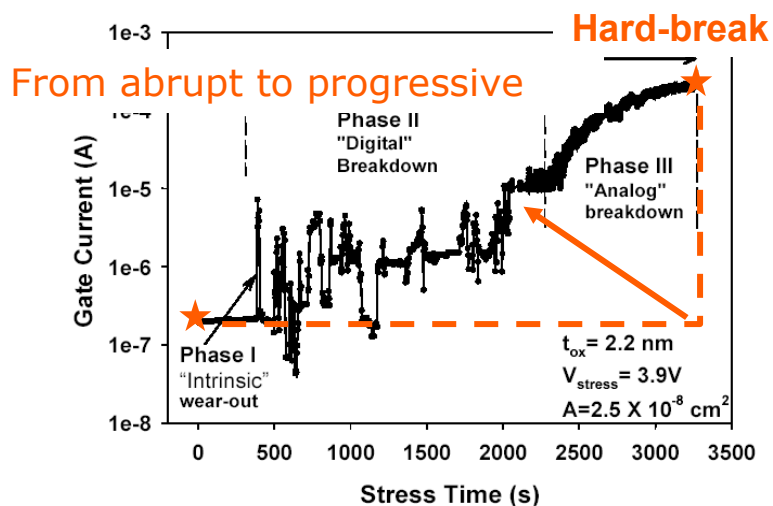
Wear-out and breakdown model for dielectric breaks
